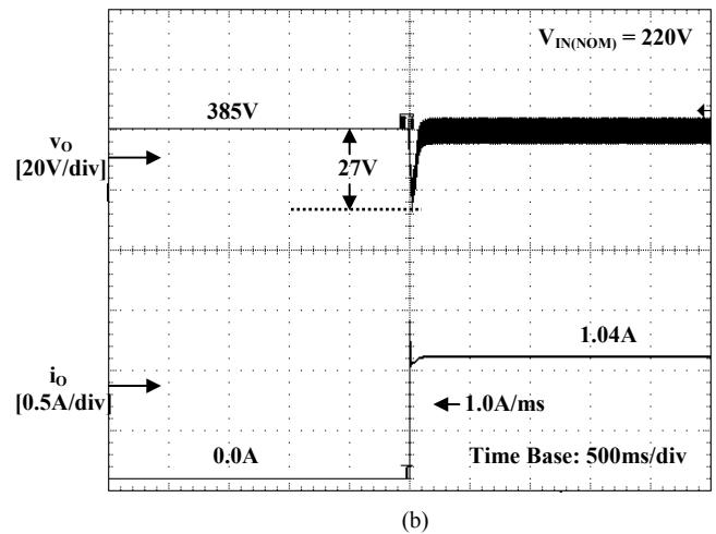
Fig. 6 Voltage undershoot for no-load-to-full-load transient at V_{IN(NOM)} = 220V (a) without voltage regulation-band control; (b) with voltage regulation-band control.
