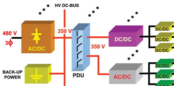
Fig. 10 High-voltage dc-bus data center power system.
