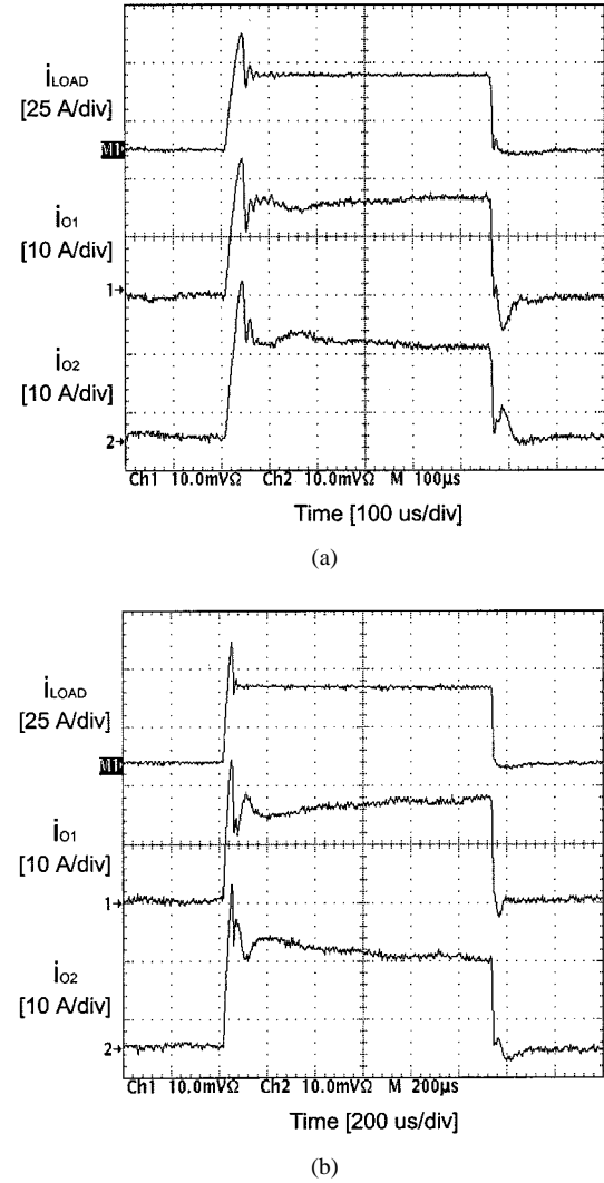
Fig. 12. Measured response of two paralleled VRMs to the dynamic load: (a) 1-kHz current-sharing loop bandwidth and (b) 300-Hz current-sharing loop bandwidth.
